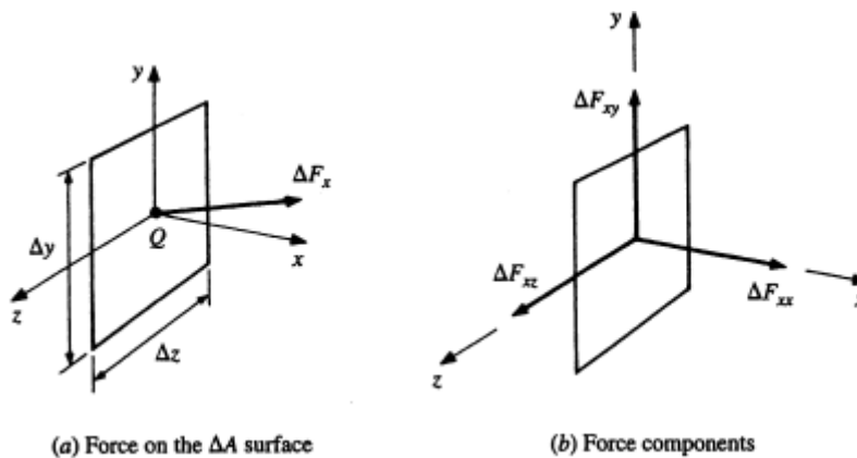
Figure 2.9.4. (a) Force on the \Delta A surface, (b) Force components
