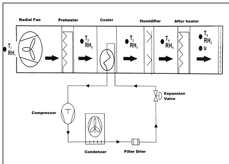
Figure 2.1.5. Schematic view of the experimental set-up.
