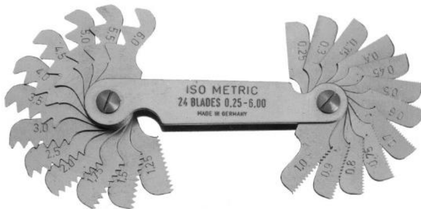
Figure 2.4.9. Threading gauge
