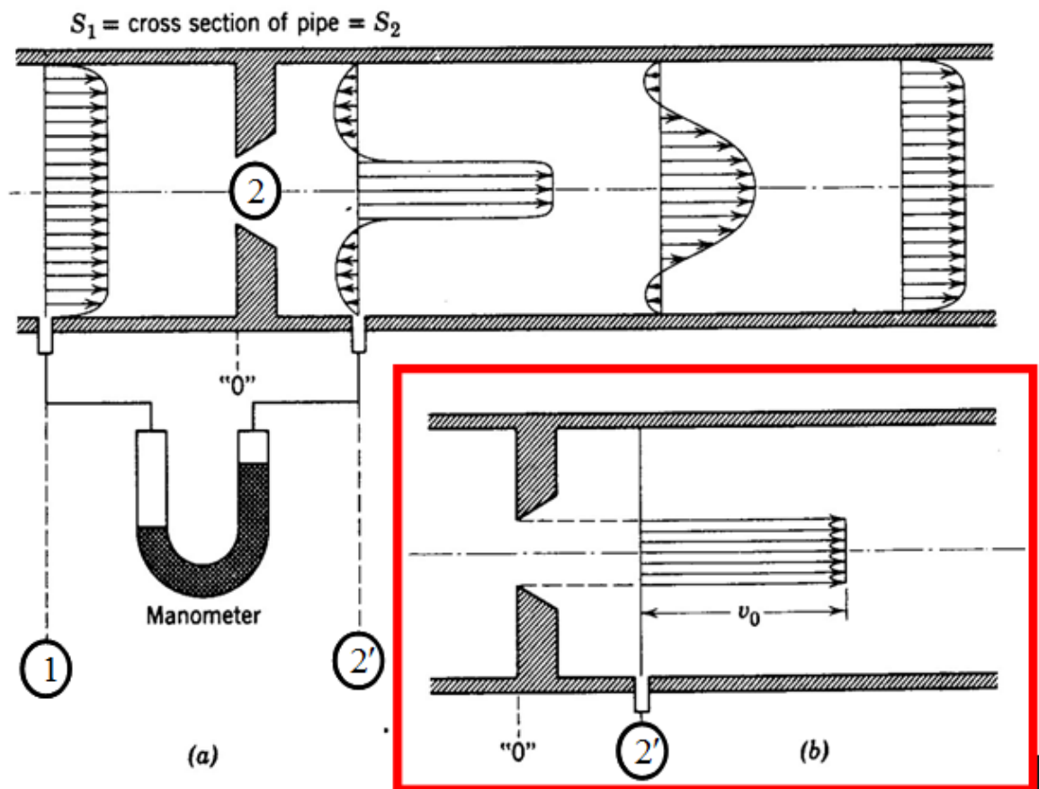
Figure 2.2.7. (a) The approximate velocity profiles at several planes near a sharp-edged orifice plate. Note: the jet emerging from the hole is somewhat smaller than the hole itself; in highly turbulent flow the jet necks down to a minimum cross section at the vena contracta. Note that there is some backflow near the wall. (b) It is assumed that the velocity profile at ② is given by the approximate profile shown. It is also assumed that the velocity profile at ① is uniform. From boundary layer theory, the pressure of the plug flow at ② is transmitted across the (assumed stagnate) interval from the plug to the pressure port
