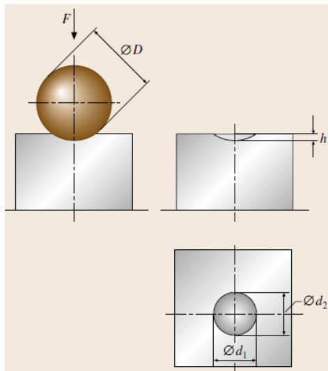
Figure 2.3.1. Principle of Brinell hardness test
