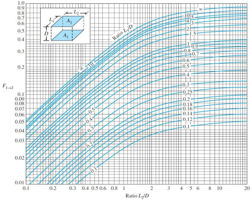
Figure 2.5.17. View factor between two aligned parallel rectangles of equal size.
