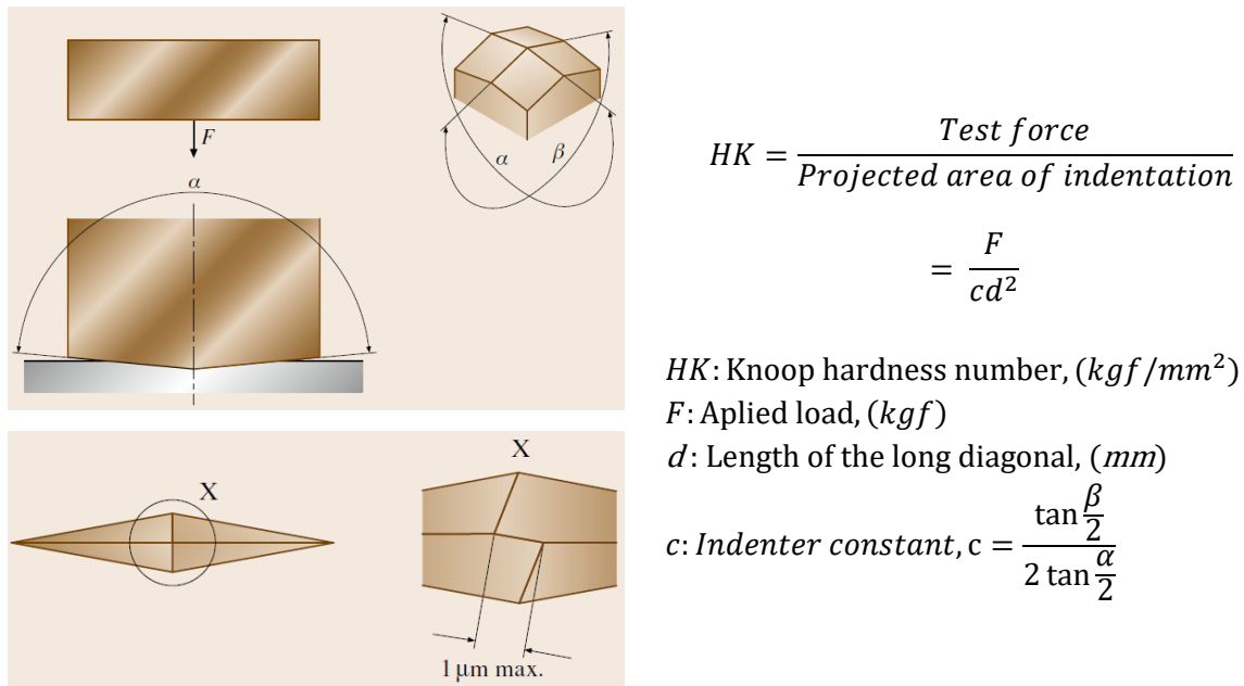
Figure 2.3.4. Principle of Knoop hardness test
