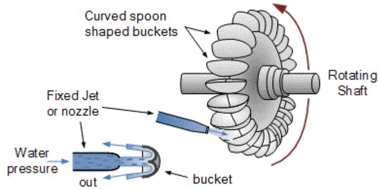
Figure 2.6.3. Configuration of water flow in buckets
