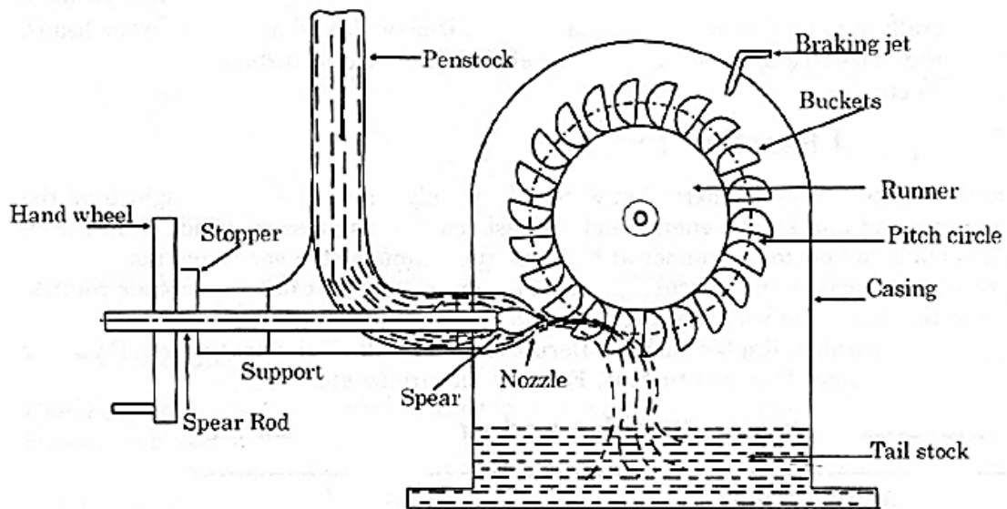
Figure 2.6.2. Schematic diagram of a Pelton Turbine
