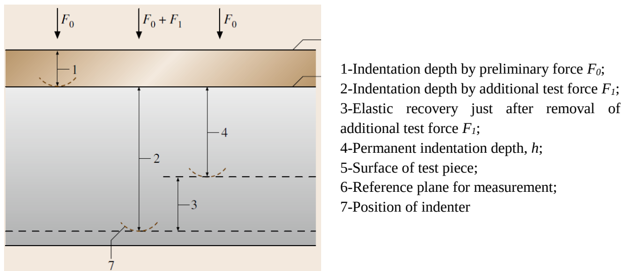
Figure 2.3.2. Principle of Rockwell hardness test
