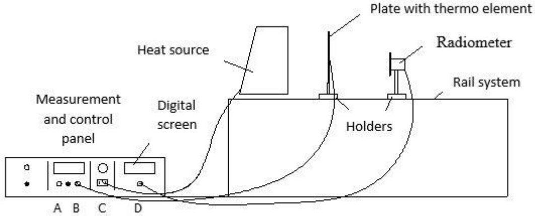
Figure 2.5.11. The experimental setup
