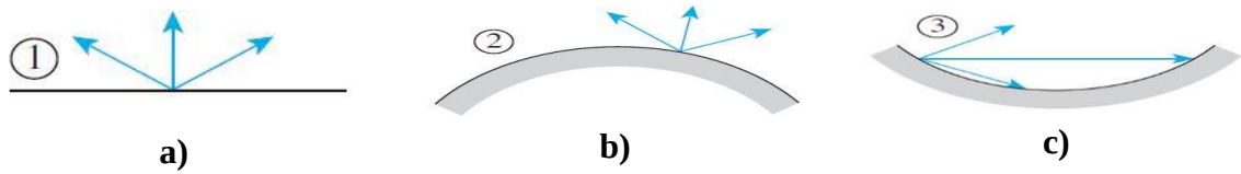
Figure 2.5.5. The view factor from a surface to itself for (a) plane surface F_{11} = 0 , (b) convex surface F_{22} = 0 , and (c) concave surface F_{33} \neq 0
