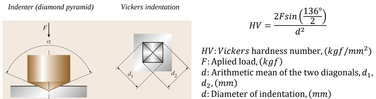
Figure 2.3.3. Principle of Vickers hardness test
