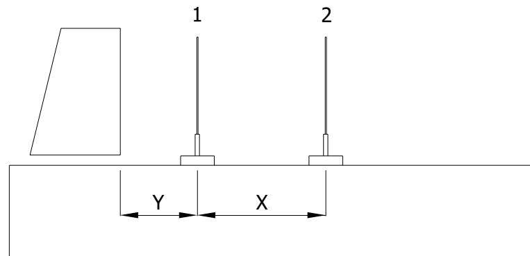
Figure 2.5.15. The positions of the plates for view factor experiment
