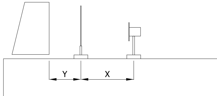
Figure 2.5.14. The positions of the radiometer and the plate
