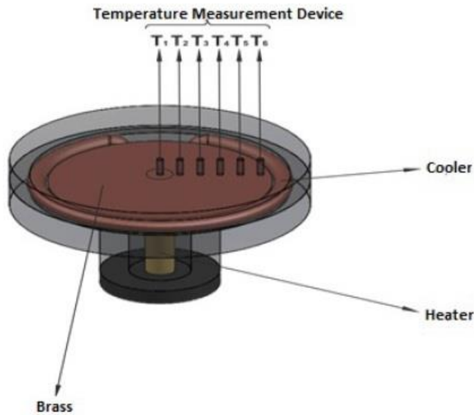
Figure 2.4.5. Radial Heat Conduction Experiment Setup
