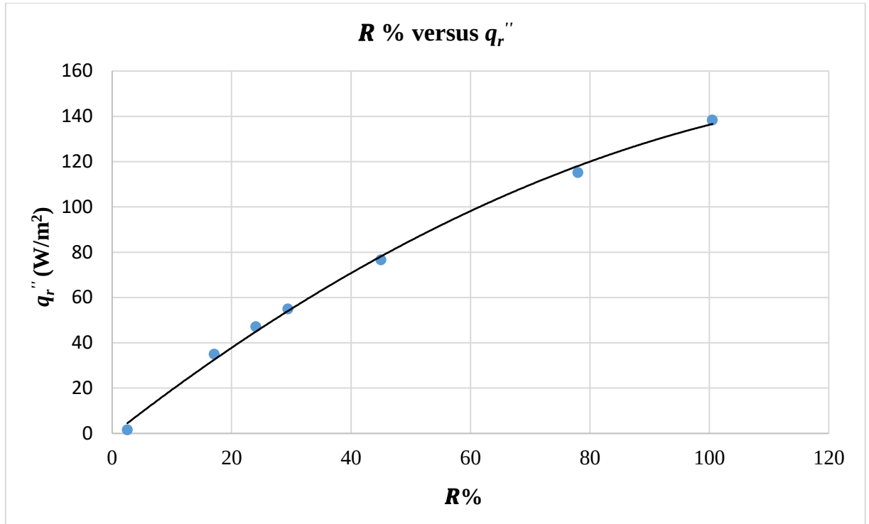
Figure 2.5.13. The relationship between the thermal radiation received by radiometer and R %.
