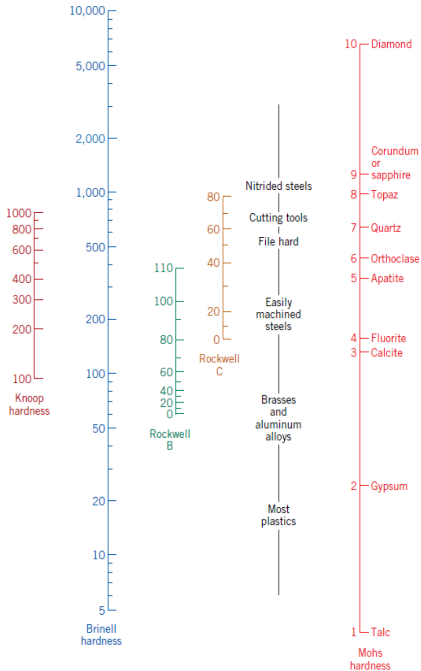
Figure 2.3.5. Comparison of several hardness scales
