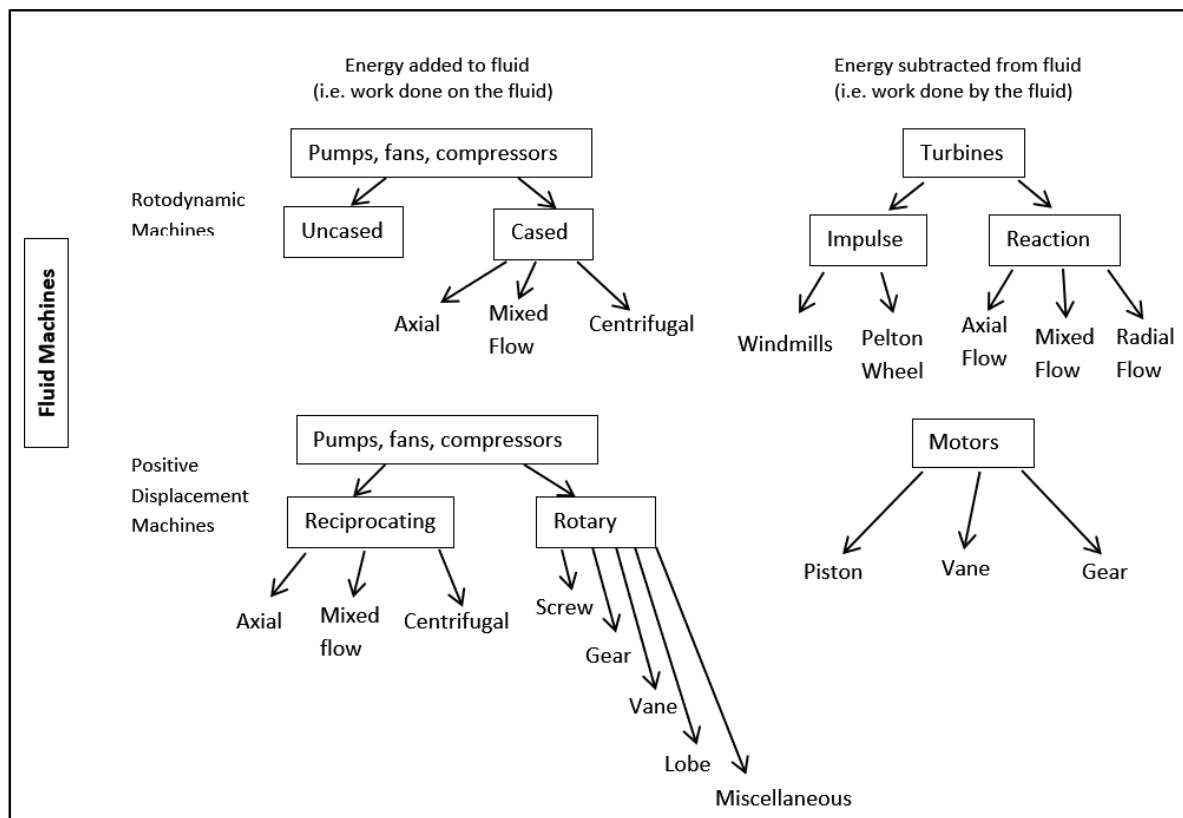
Figure 2.7.1. Classification of fluid machines
