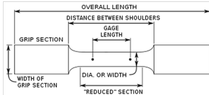
Figure 2.3.6. Test specimen
