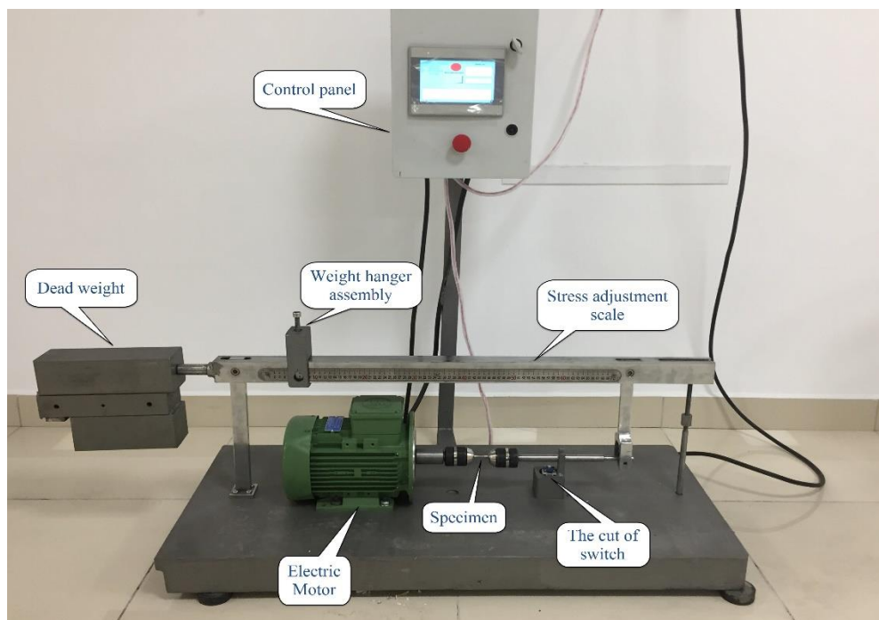
Figure 2.8.9. Rotating-bending fatigue testing apparatus ant its components
