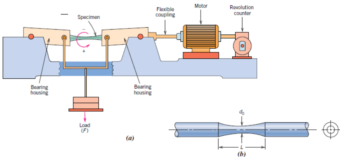
Figure 2.8.1. For rotating-bending fatigue tests, schematic diagrams of (a) a testing apparatus, and (b) a test specimen.
