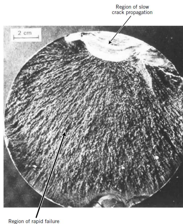
Figure 2.8.5. Fatigue failure surface
