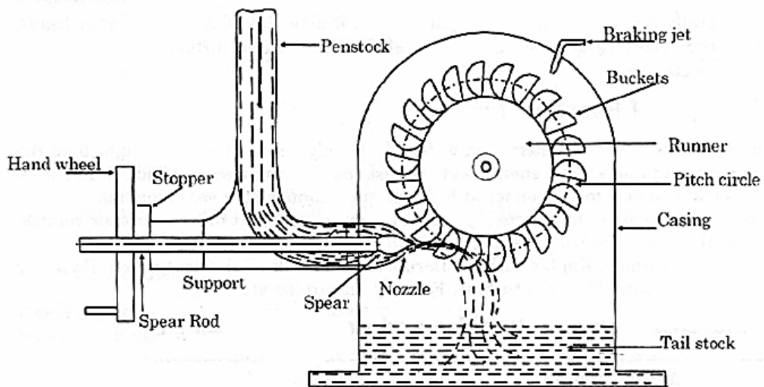
Figure 2.7.2. Schematic diagram of a Pelton turbine
