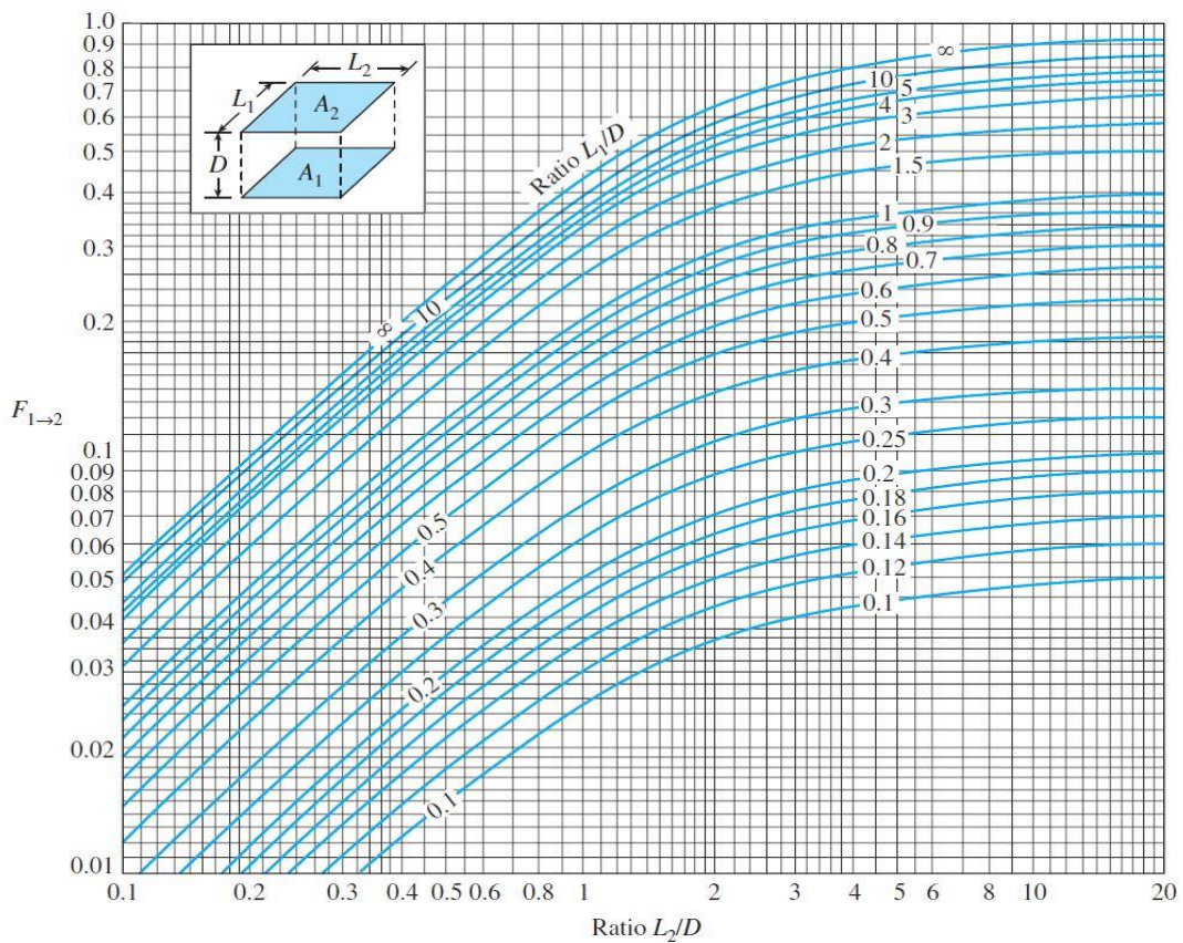
Figure 2.9.17. View factor between two aligned parallel rectangles of equal size.
