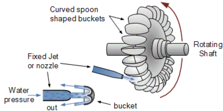
Figure 2.7.3. Configuration of water flow in buckets
