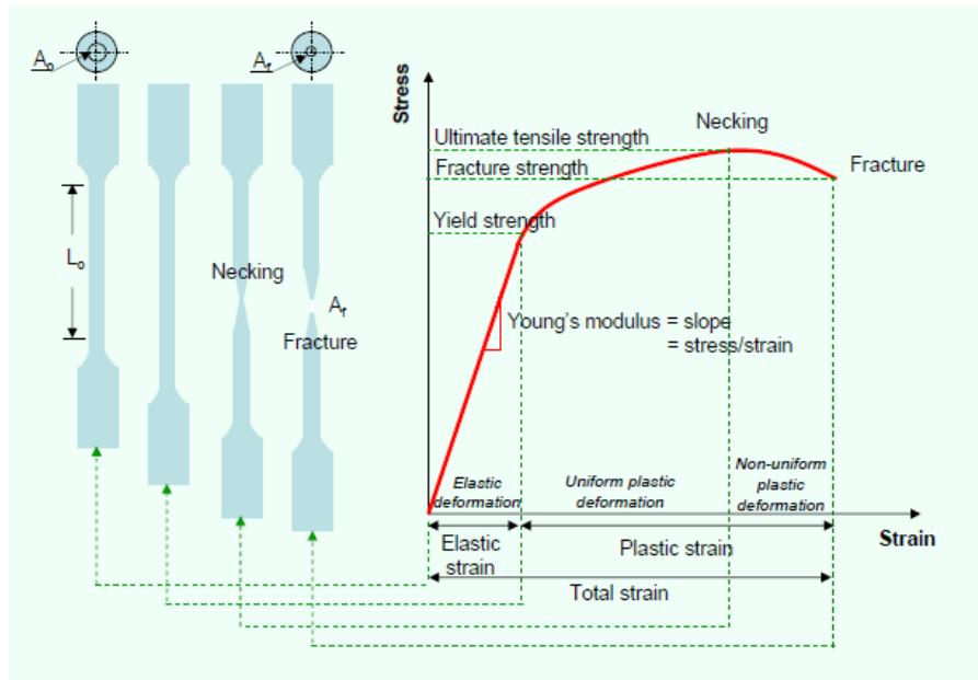
Figure 2.3.2. Stress-strain curve
