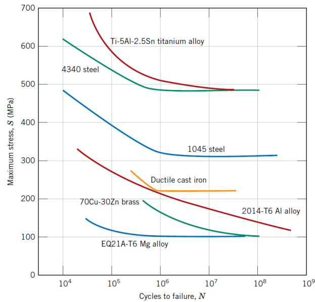
Figure 2.8.3. Maximum stress versus logarithm of the number of cycles to fatigue failure for seven metal alloys.
