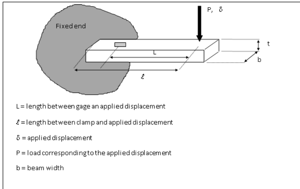
Figure 2.1.10. Beam with strain gage in flexure fixture
