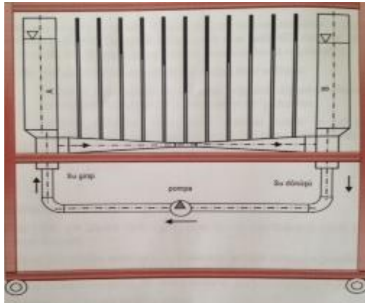
Figure 2.2.3. Experimental setup
