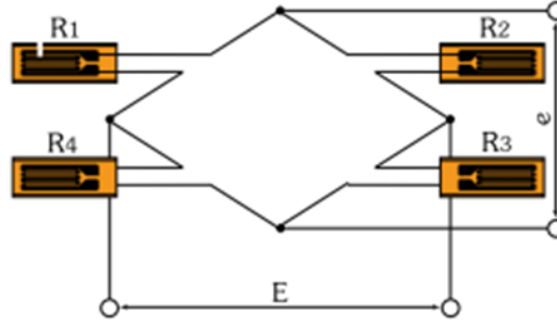
Figure 2.1.9. Full Wheatstone bridge
