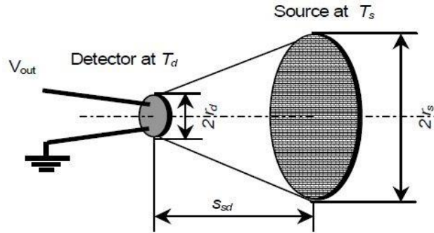
Figure 2.9.12. The circular detector (radiometer) and the circular source
