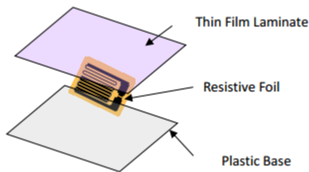
Figure 2.1.1. Strain gauge construction
