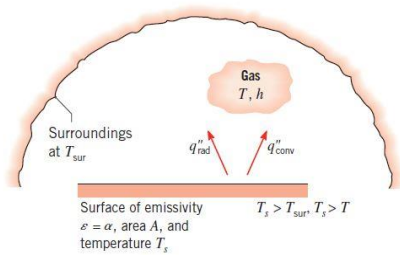
Figure 2.9.9. Radiation heat transfer from a gray surface
