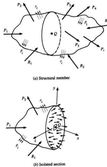
Figure 2.1.2. (a) Structural member and (b) Isolated section
