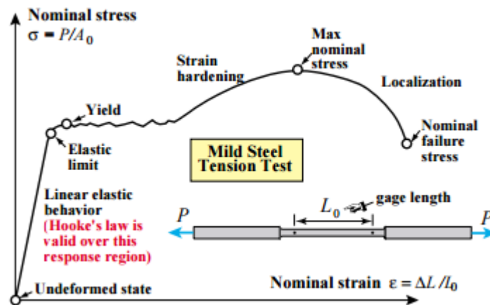
Figure 2.1.5. Stress vs strain diagram
