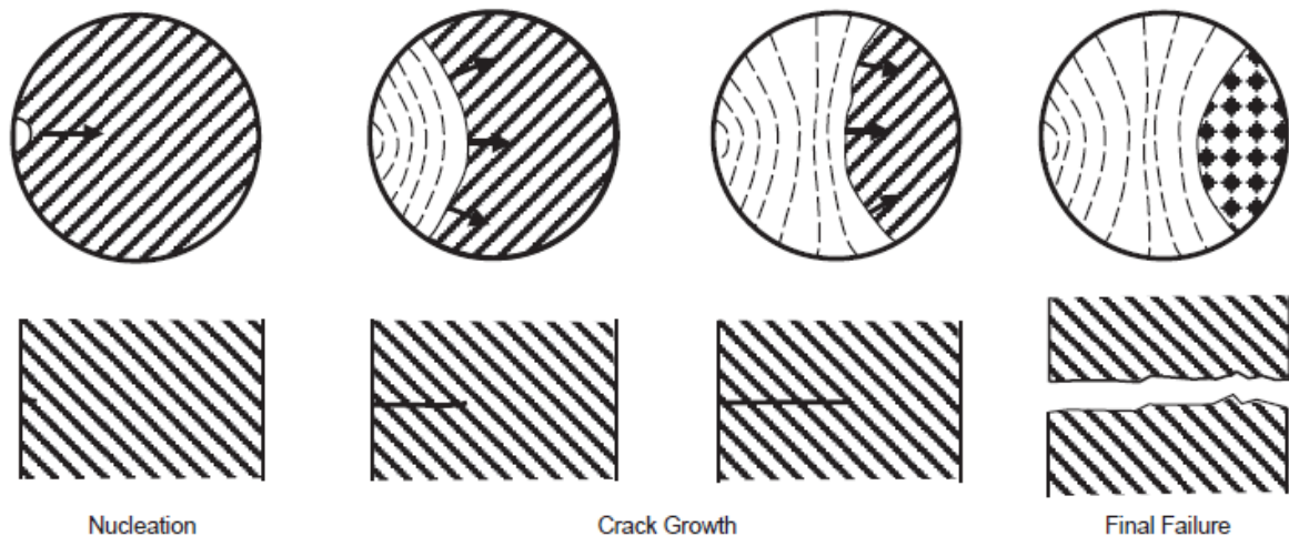
Figure 2.8.4. Typical propagation of a fatigue crack
