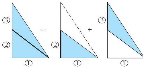
Figure 2.9.7. The view factor from a surface to a composite surface
