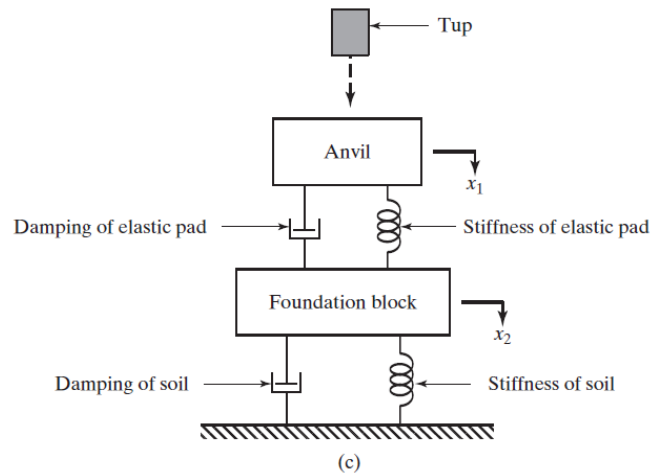
Figure 2.5.8. Vibration model of a forging hammer
