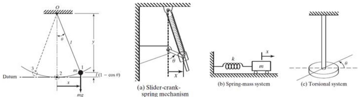
Figure 2.5.3. Basic single degree-of-freedom systems
