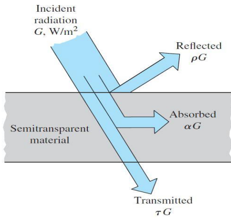
Figure 2.9.4. The absorption, reflection, and transmission of incident radiation by a semitransparent material
