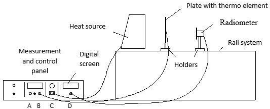
Figure 2.9.11. The experimental setup
