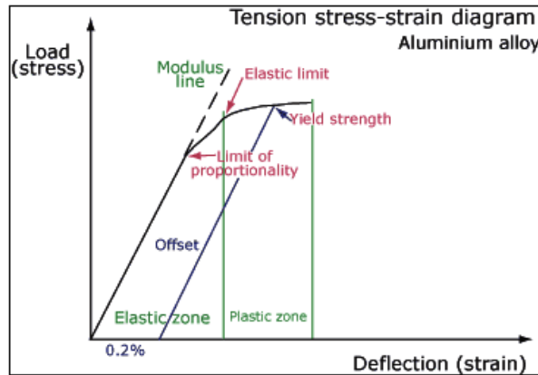
Figure 2.3.4. Stress-strain curve
