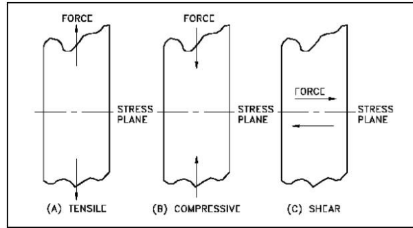
Figure 2.3.1. Types of stresses
