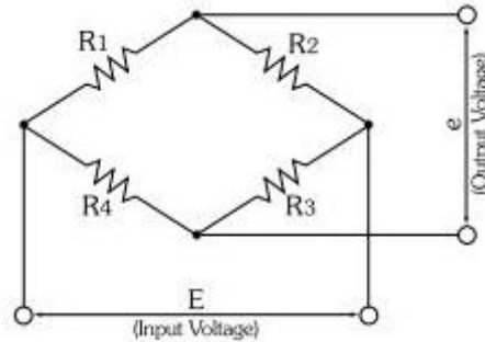
Figure 2.1.6. Wheatstone bridge
