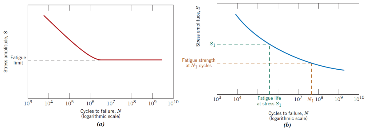
Figure 2.8.2. Stress amplitude ( S ) versus logarithm of the number of cycles to fatigue failure ( N ) for (a) a material that displays a fatigue limit and (b) a material that does not display a fatigue limit.
