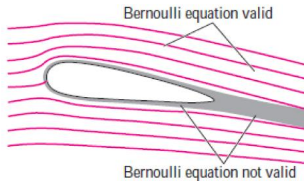
Figure 2.2.1. Practicable regions of Bernoulli equation
