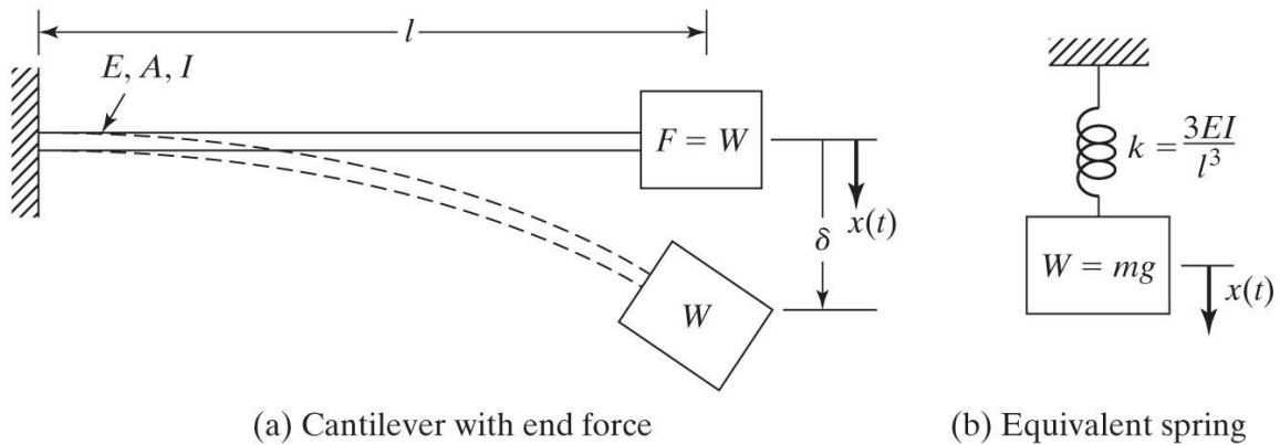
Figure 2.5.9. Cantilever beam and its equivalent spring model
