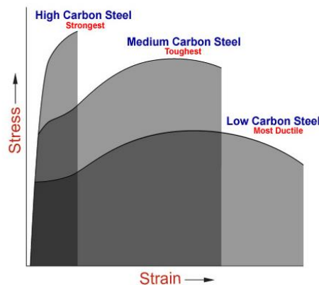
Figure 2.3.5. Toughness of the materials
