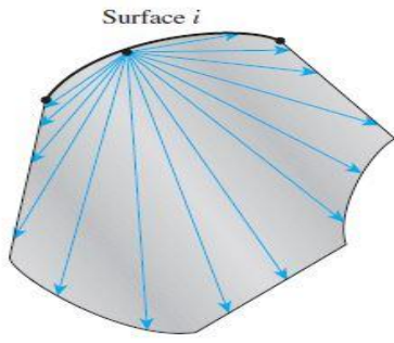
Figure 2.9.6. The radiation leaving any surface i of an enclosure
