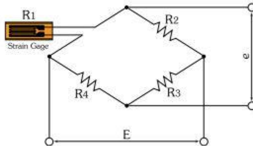
Figure 2.1.7. Quarter Wheatstone bridge
