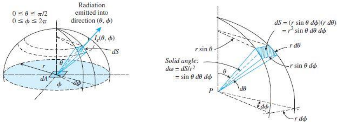
Figure 2.9.3. The emission of radiation from a differential surface element into the surrounding hemispherical space through a differential solid angle
