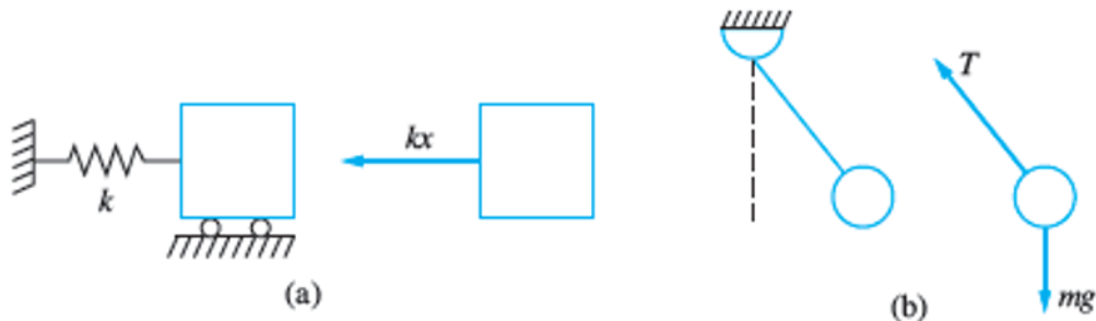
Figure 2.5.1. (a) When the block is displaced from equilibrium, the force developed in the spring (as a result of the stored potential energy) pulls the block back toward the equilibrium position (b) When the pendulum is rotated away from the vertical equilibrium position, the moment of the gravity force about the support pulls the pendulum back toward the equilibrium position
