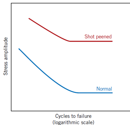
Figure 2.8.8. Schematic S – N fatigue curves for normal and shot-peened steel.
