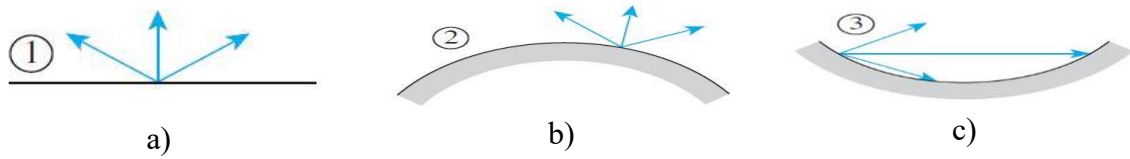
Figure 2.9.5. The view factor from a surface to itself for (a) plane surface F_{11} = 0 , (b) convex surface F_{22} = 0 , and (c) concave surface F_{33} \neq 0
