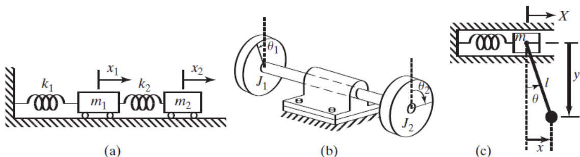
Figure 2.5.4. Typical second degree-of-freedom systems
