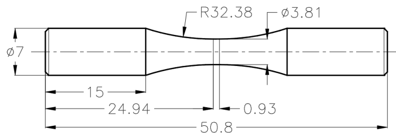
Figure 2.8.10. Dimensions of fatigue life test specimen
