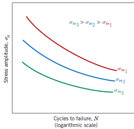
Figure 2.8.6. Demonstration of the influence of mean stress \sigma_m on S–N fatigue behavior.
