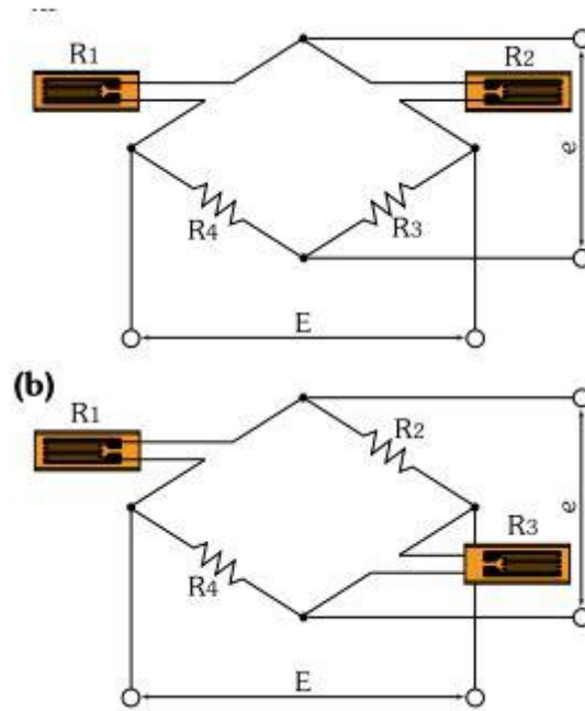
Figure 2.1.8. Half Wheatstone bridge
