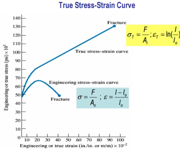
Figure 2.3.3. True stress-strain curve
