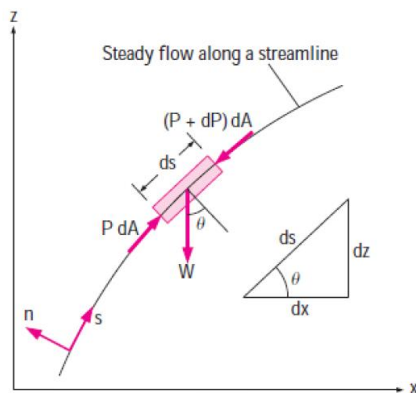
Figure 2.2.2. The forces acting on a fluid particle along a streamline
