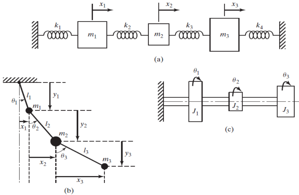
Figure 2.5.5. Representative examples three degree-of-freedom systems
