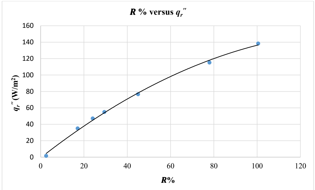
Figure 2.9.13. The relationship between the thermal radiation received by radiometer and R %.
