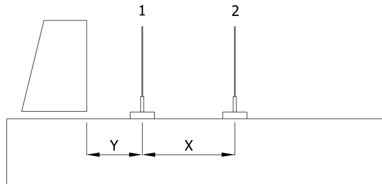
Figure 2.9.15. The positions of the plates for view factor experiment
