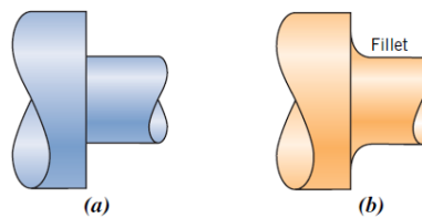
Figure 2.8.7. Demonstration of how design can reduce stress amplification.
