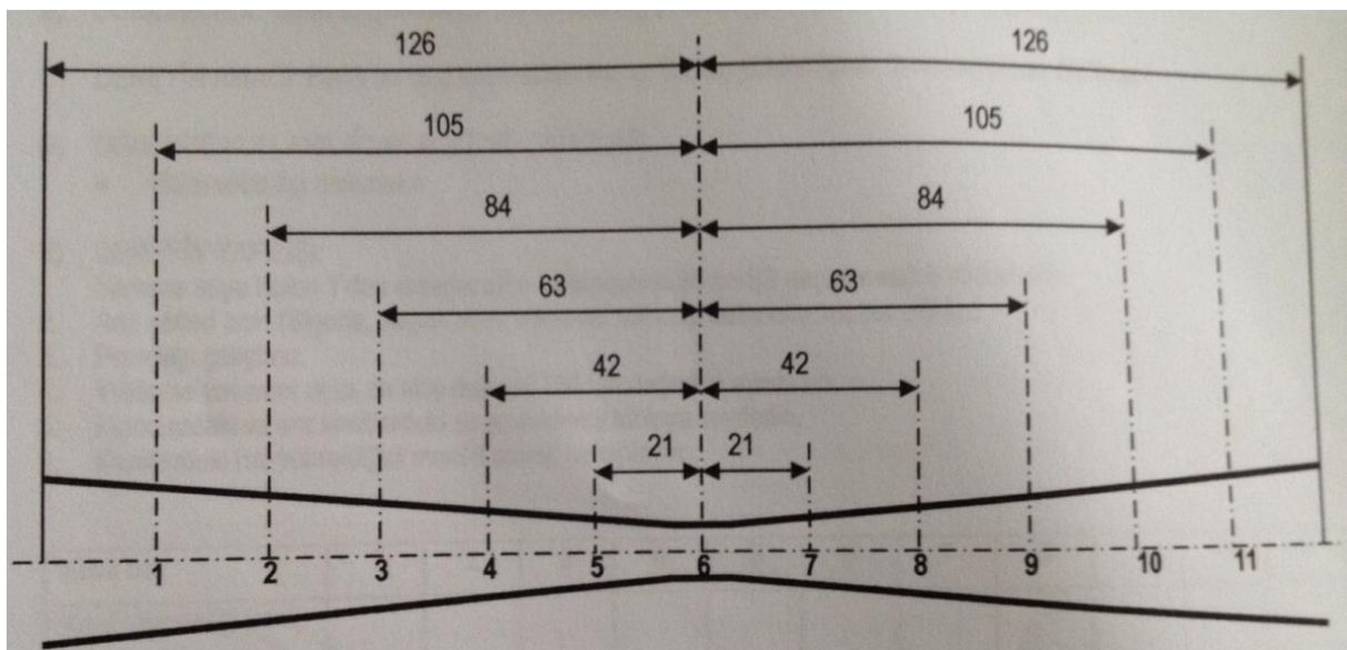
Figure 2.2.4. Front view of main tube
