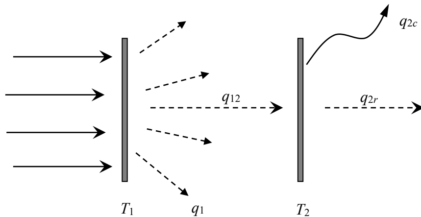
Figure 2.9.16. Heat transfer from plates
