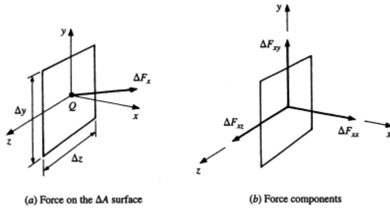
Figure 2.1.3. (a) Force on the \Delta A surface, (b) Force components
